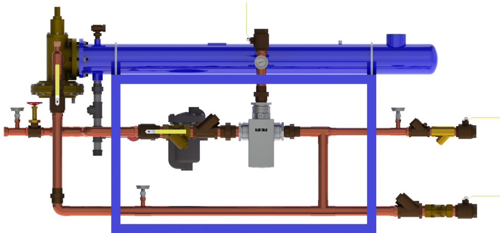
Flo-Rite-Temp® FRT66550 Single Wall Instantaneous Water Heater
